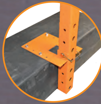
Adjustable Hinge Plate & Post
